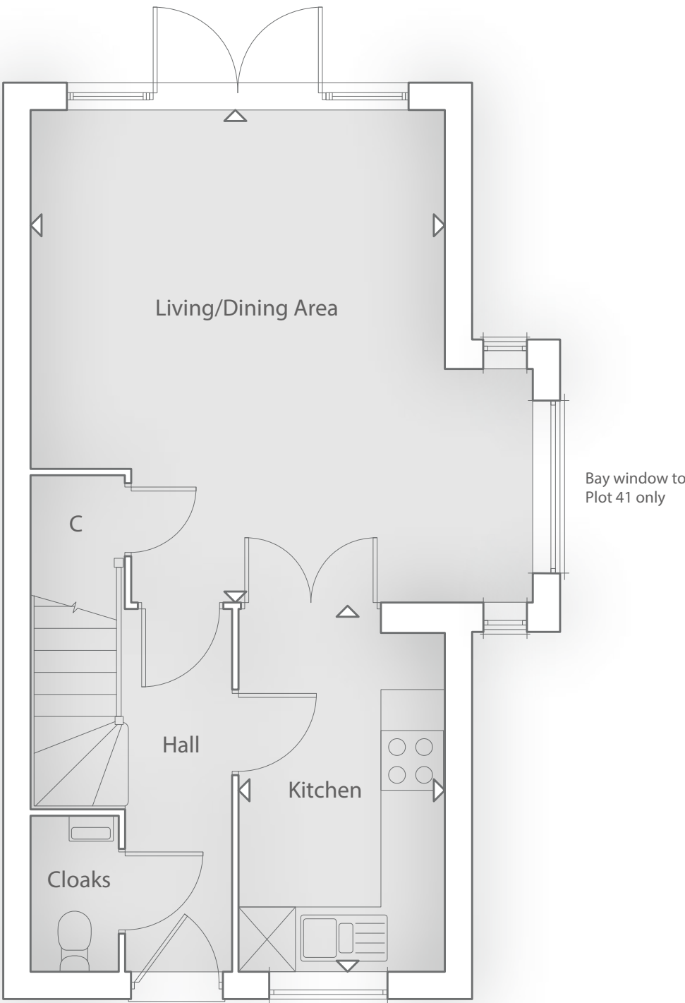
GROUND FLOOR
