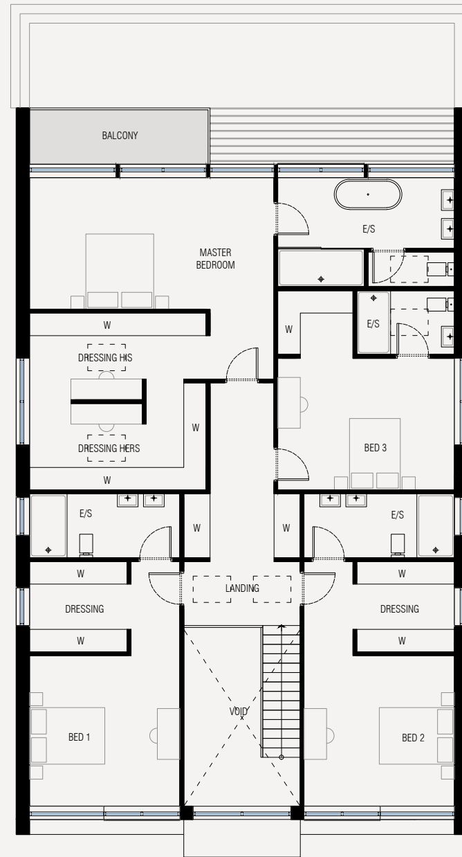
02 First Floor Plan - House 1
